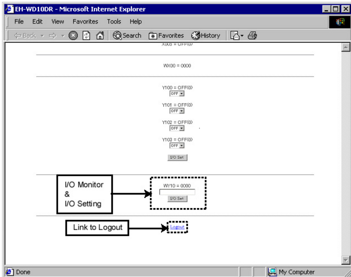
Figure 5.11 d_mobile.htm
