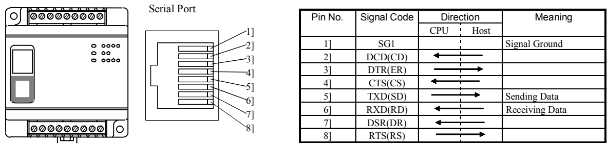
Figure 3.3 Serial Port Circuit Diagram and Pin Numbers
