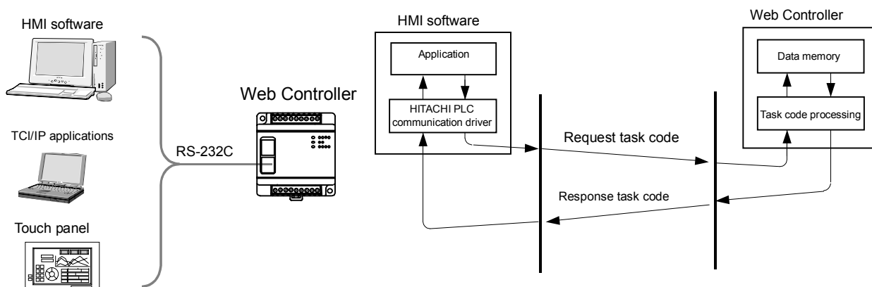
Figure 10.10 Serial port Passive HIProtocol
