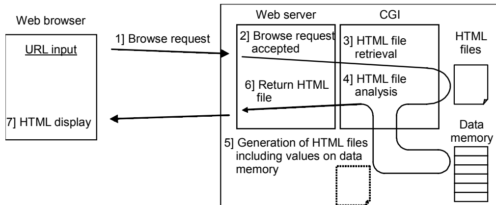
Figure 6.7 Reading out the values of I/O memory via a Web browser
