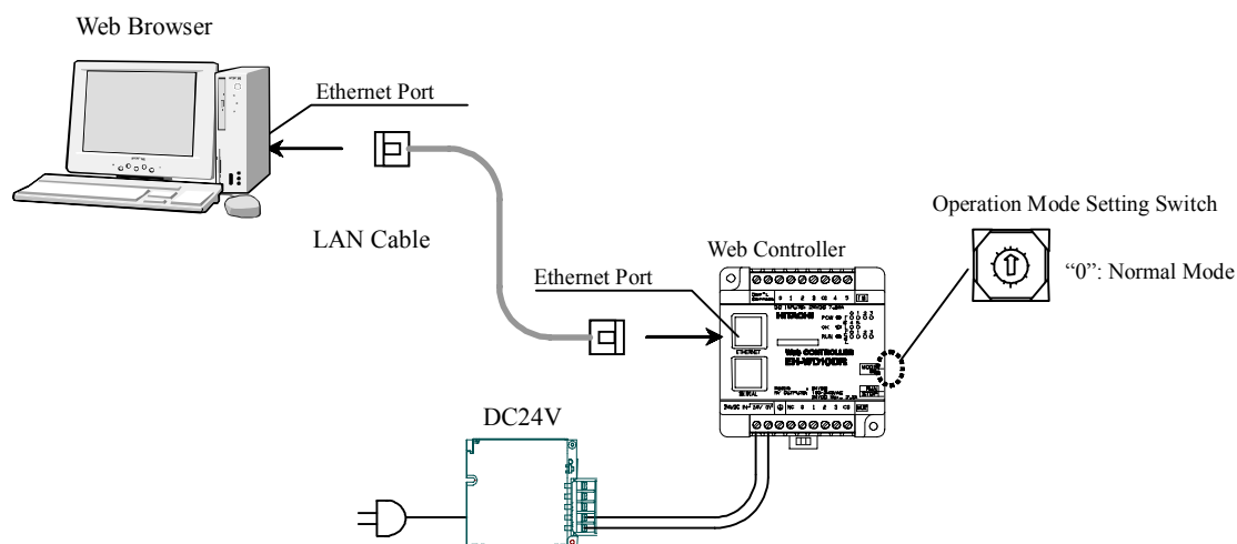
Figure 4.1 Sample Connections
