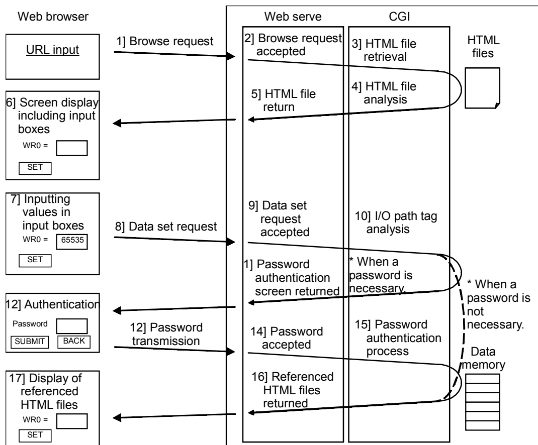
Figure 6.8 Setting values on I/O memory via a Web browser
