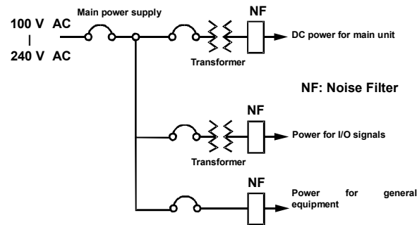
Figure 17.4 Example of power system diagram
