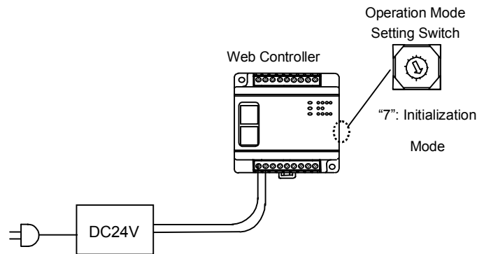
Figure Appendix 2.1 Setting Switch during Initialization Mode
