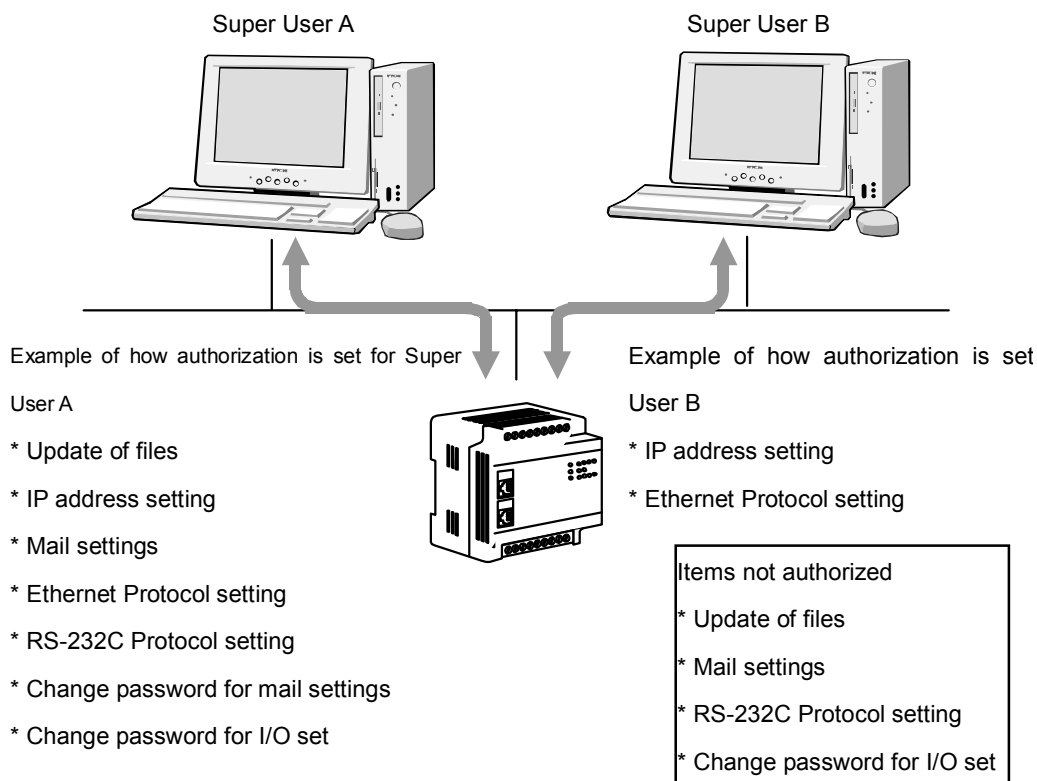
Figure 1.13 Sample setting of privileges for each Super User
