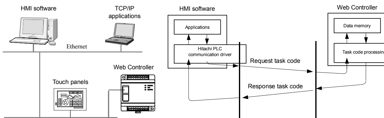
Figure 9.1 Composition of task code communication equipment
