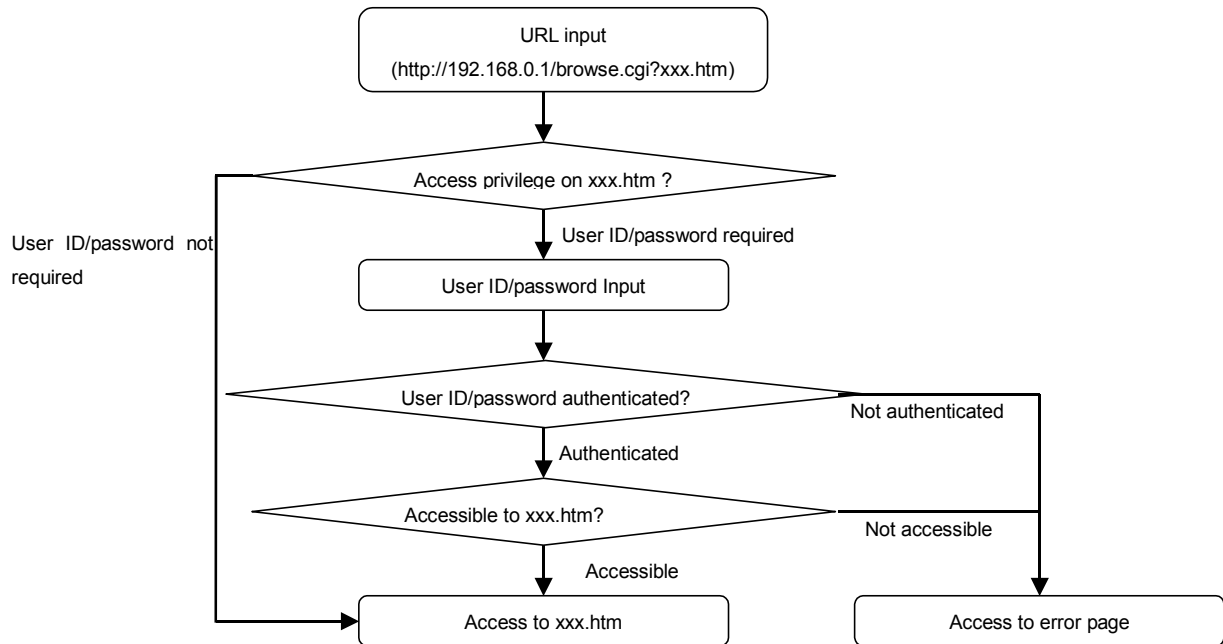
Figure 6.5 Access flow chart
