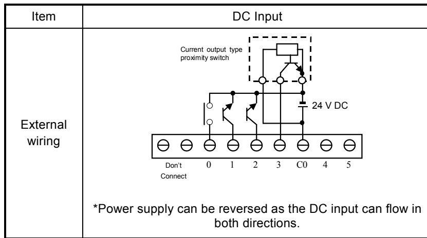
Figure 17.7 Input wiring
