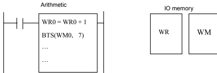
Figure 1.5 Arithmetic operation function
