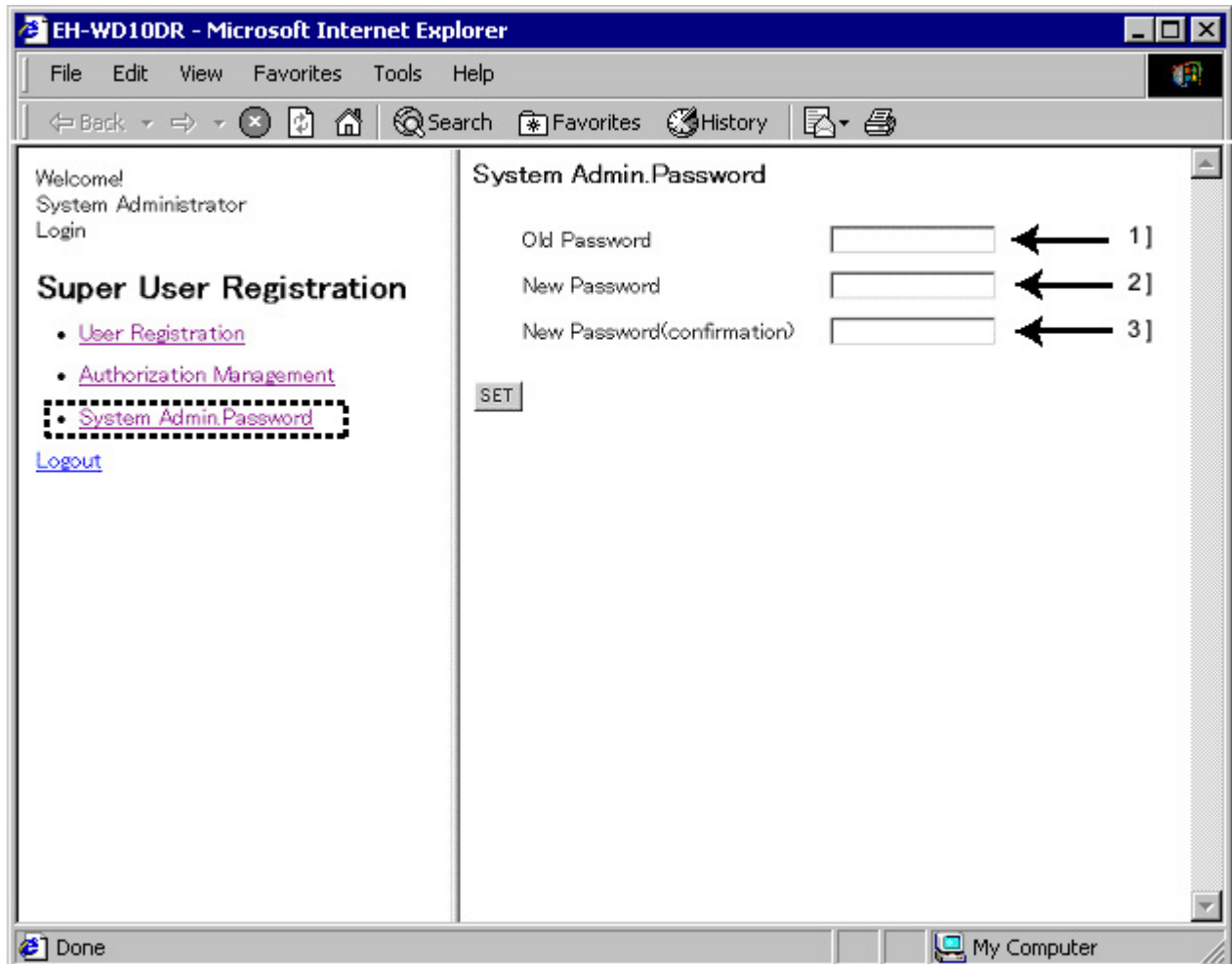
Figure 12.5 Screen composition of System Admin.Password
