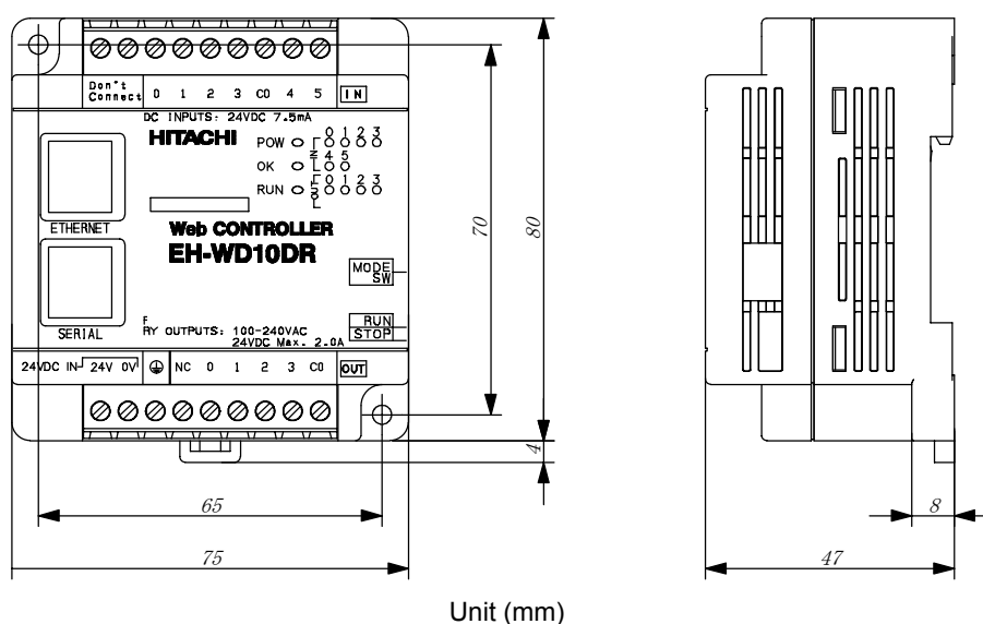
Figure 16.2 Dimensions Diagram
