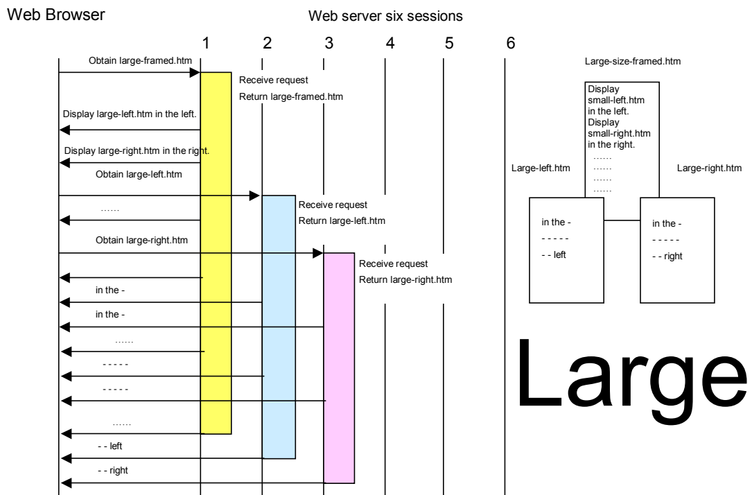
Figure 6.12 Web server – six session operation: large file size
