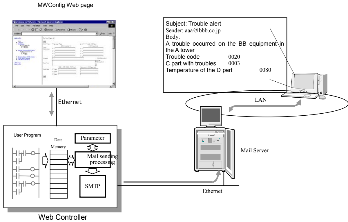
Figure 1.14 Mail sending function
