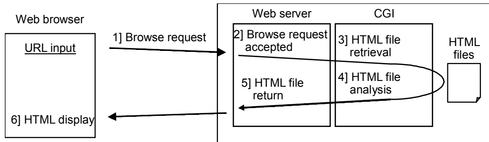
Figure 6.6 Browsing Web pages
