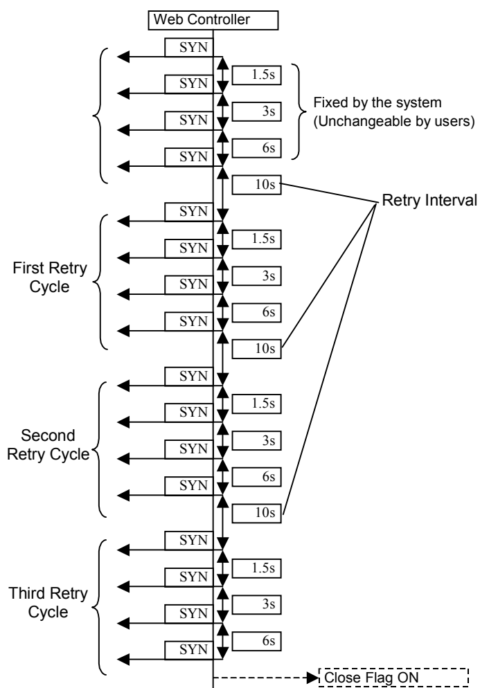
Figure 9.2 Connection Open Retry Sequence
