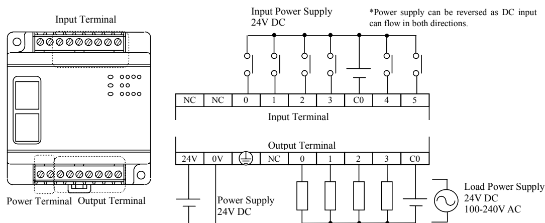
Figure 3.1 Terminals Configuration and Connection
