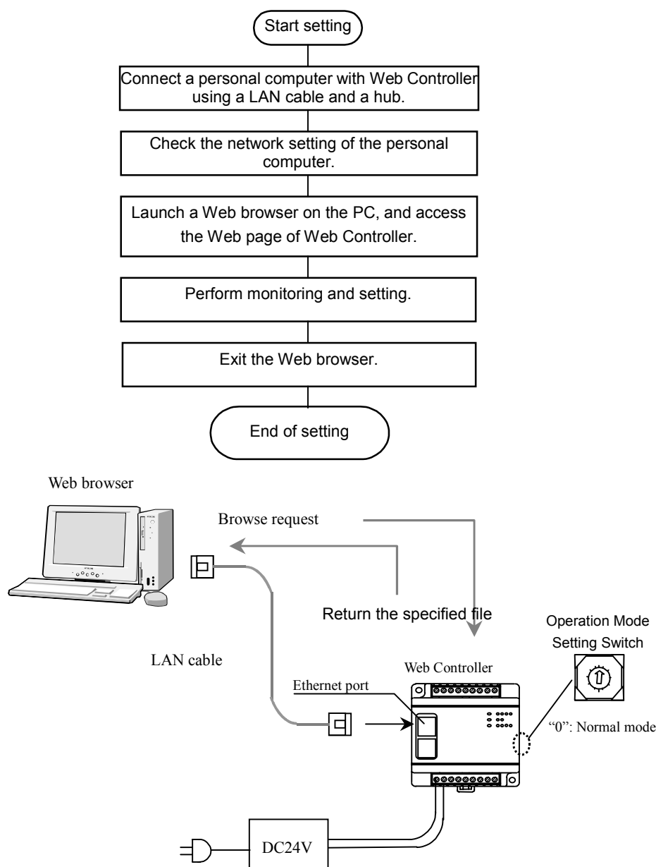
Figure 5.1 Outline of access procedures
