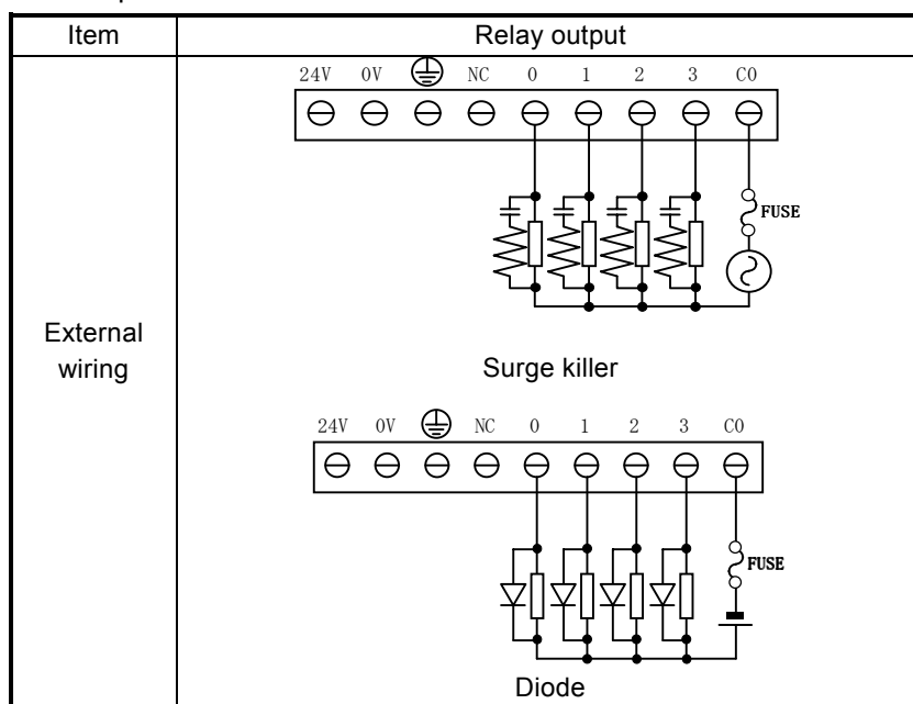
Figure 17.8 Relay output wiring
