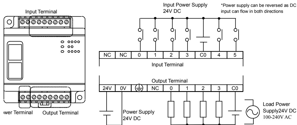
Figure 16.2 Terminals Configuration and Connection
