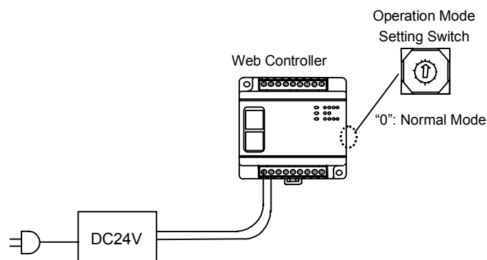
Figure Appendix 2.2 Setting Switch during the use in Normal Mode
