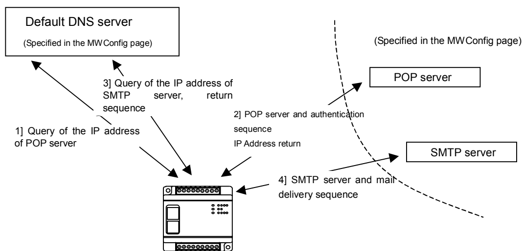
Figure 7.2 Mail sending operation
