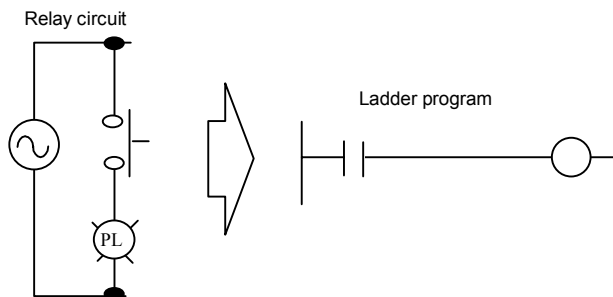
Figure 1.4 User Program
