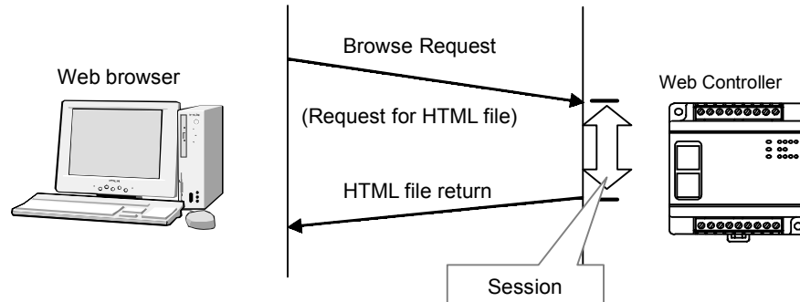
Figure 6.9 Session
