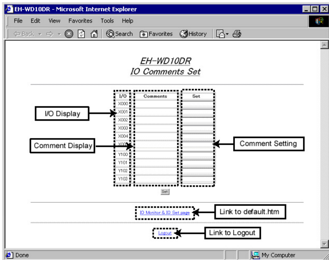
Figure 5.8 comments.htm
