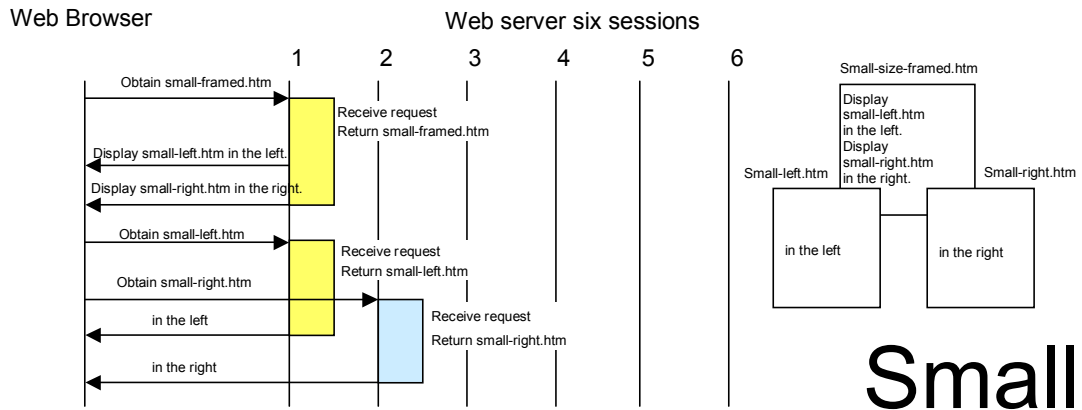
Figure 6.11 Web server – six session operation: small file size
