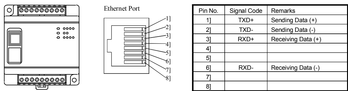
Figure 3.2 Ethernet Port Pin Numbers and Descriptions
