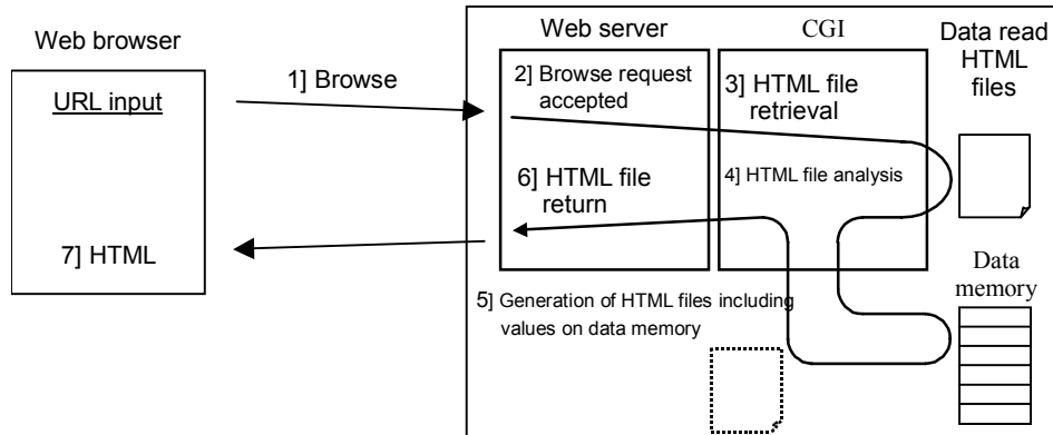
Figure 1.9 Reading out the values of data memory via a Web browser
