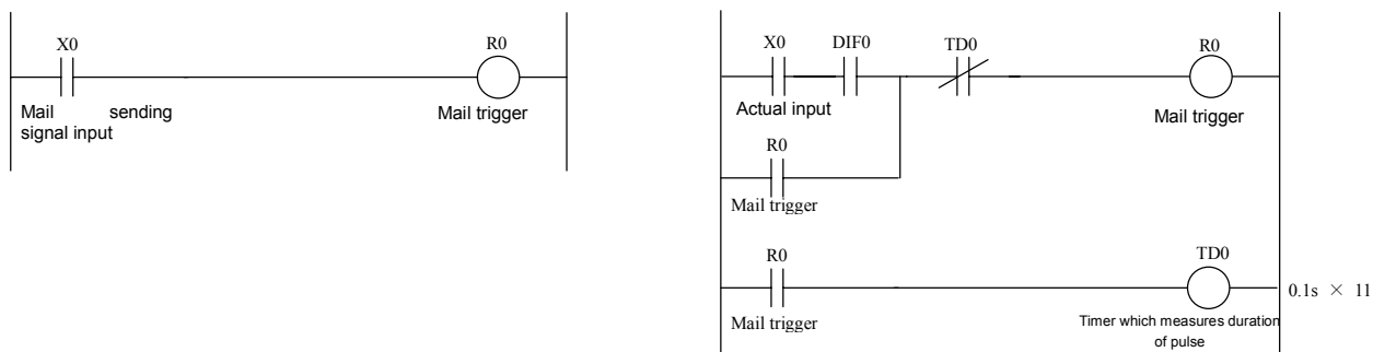
Figure 7.3 Sample user program for sending mails
