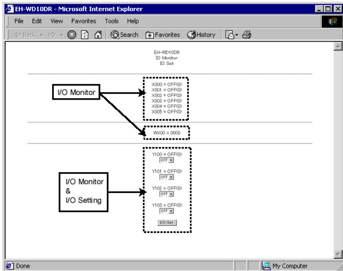
Figure 5.10 d_mobile.htm
