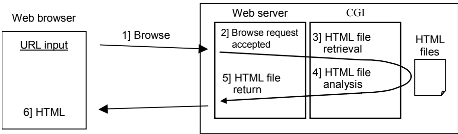
Figure 1.8Browsing Web pages
