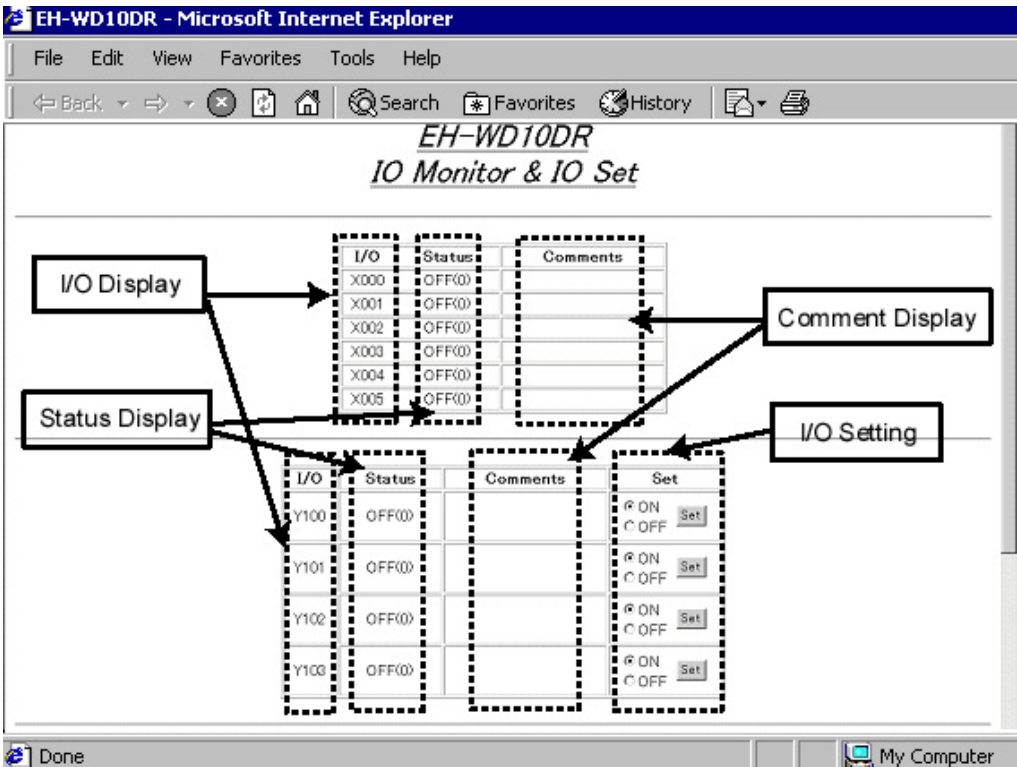
Figure 5.5 default.htm
