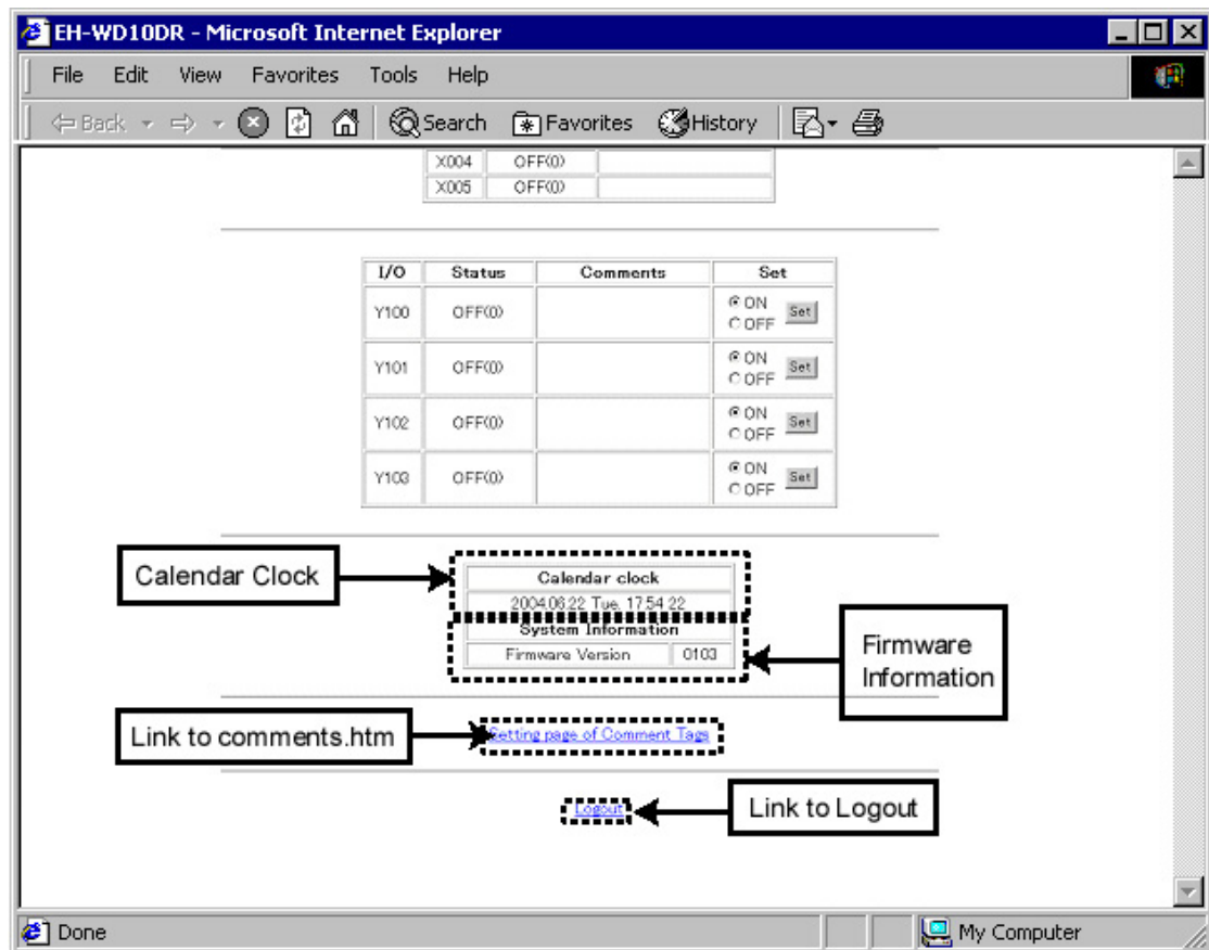
Figure 5.6 default.htm
