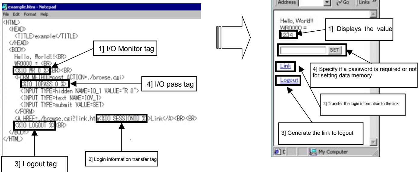
Figure 14.3 Extension tags and display examples
