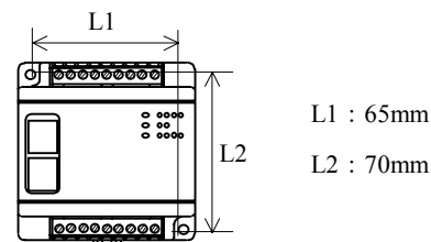
Figure 17.2 External dimensions
