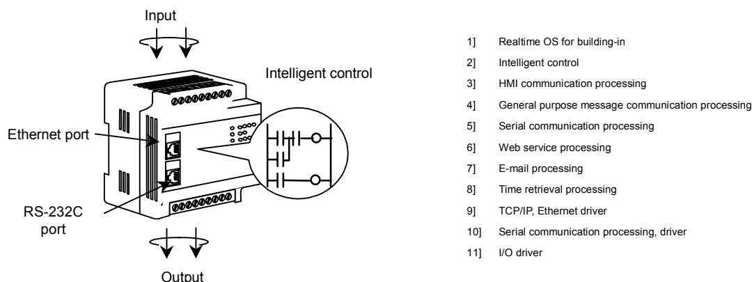
Figure 1.1 All-in-one controller
